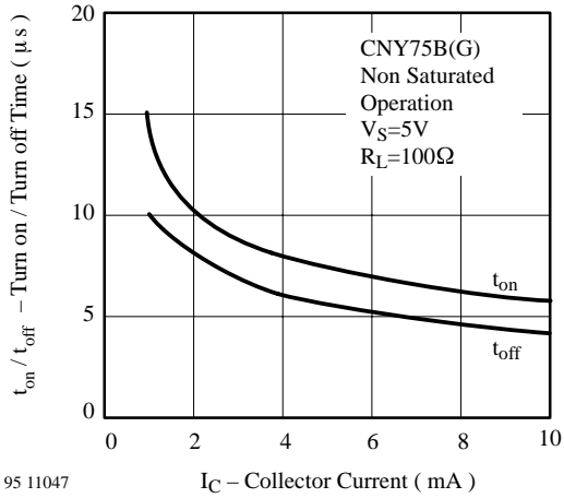
95 11047 Figure 26. Turn on / off Time vs. Collector Current
