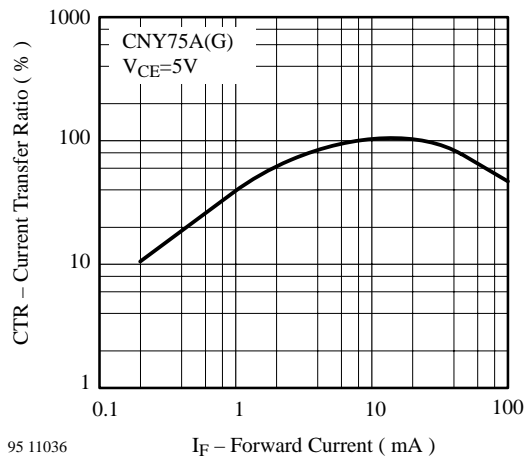
95 11036 I_F – Forward Current ( mA ) Figure 19. Current Transfer Ratio vs. Forward Current
