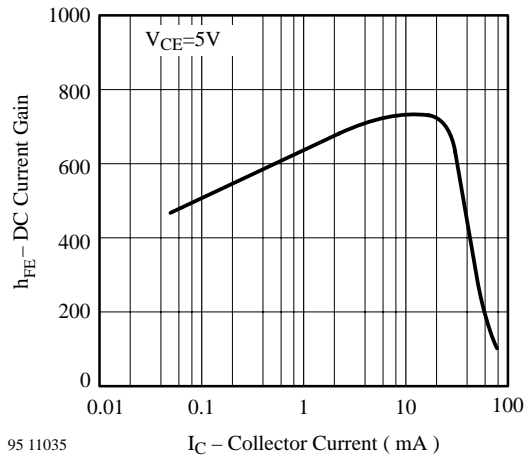
95 11035 I_C – Collector Current ( mA ) Figure 18. DC Current Gain vs. Collector Current
