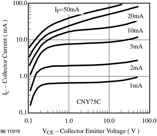
96 11919 V_{CE} – Collector Emitter Voltage ( V ) Figure 14. Collector Current vs. Collector Emitter Voltage
