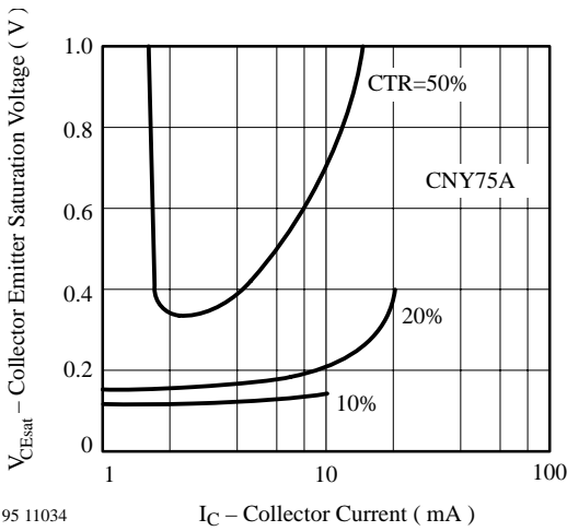
95 11034 I_C – Collector Current ( mA ) Figure 15. Coll. Emitter Sat. Voltage vs. Coll. Current
