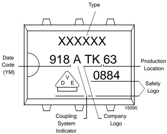
Figure 28. Marking example
