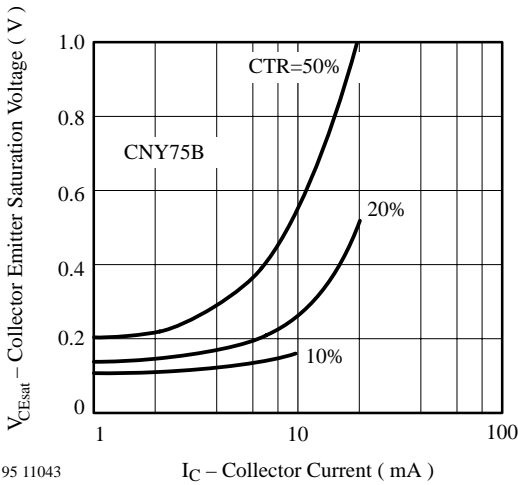
95 11043 I_C – Collector Current ( mA ) Figure 16. Coll. Emitter Sat. Voltage vs. Coll. Current
