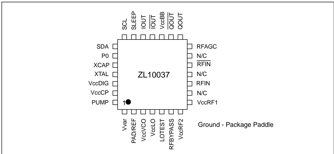
Figure 2 - Pin Diagram
