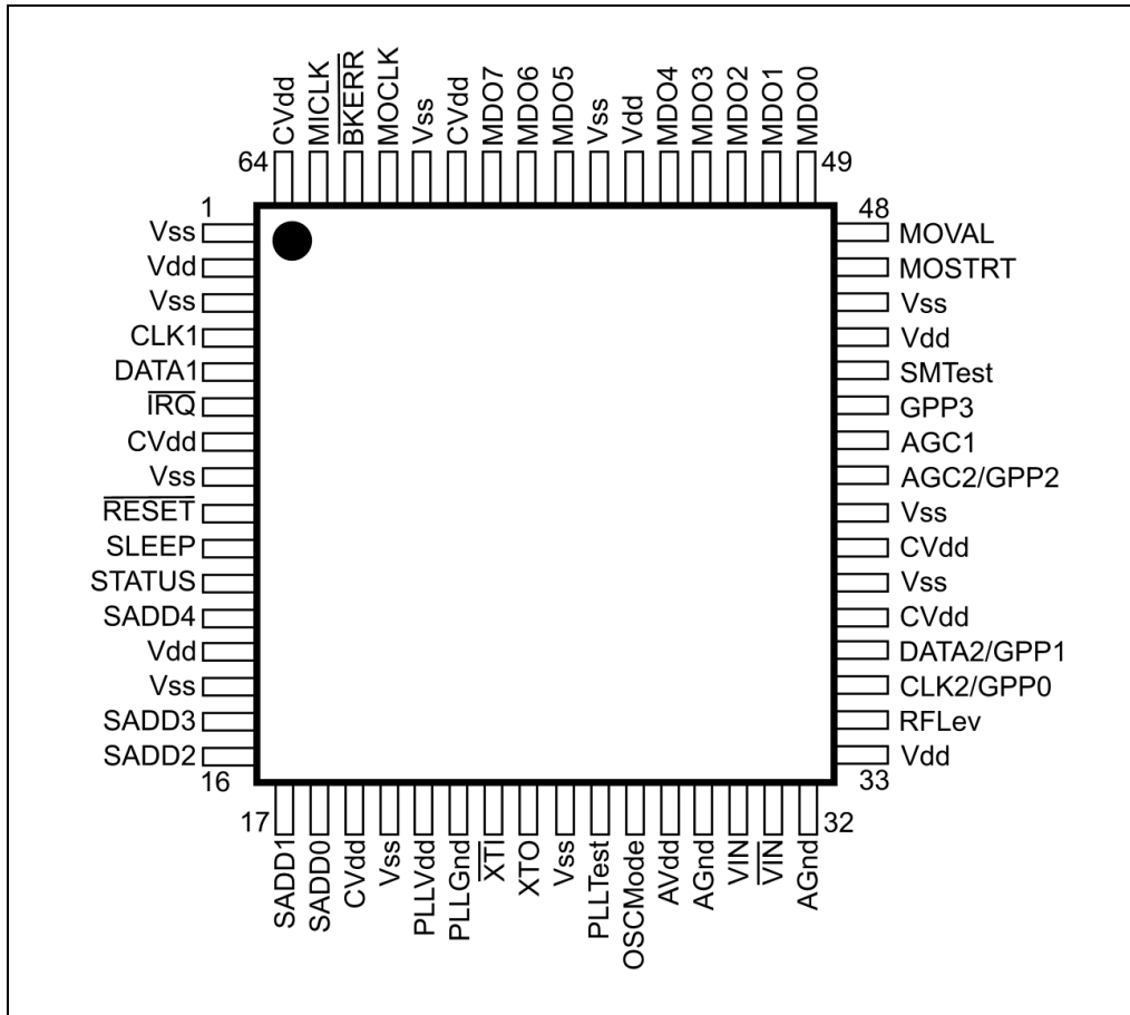
Figure 2 - Pin Outline
