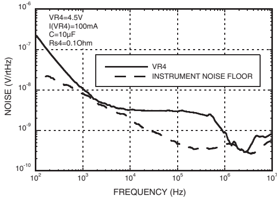
VR4 Noise Spectral Density, Vdd = 5.5V
