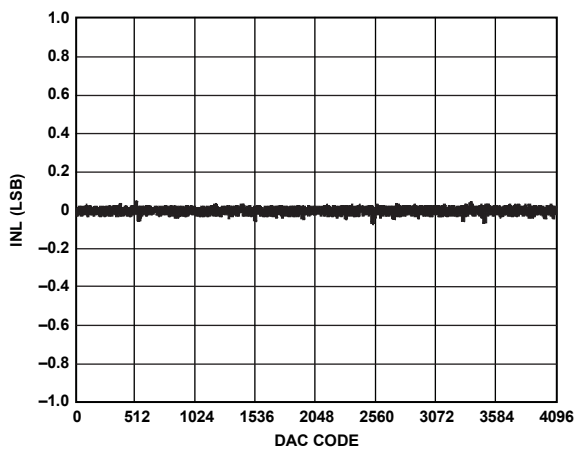
Figure 8. AD5025 INL
