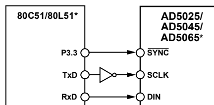
Figure 48. AD5025/AD5045/AD5065 to 80C51/80L51 Interface
