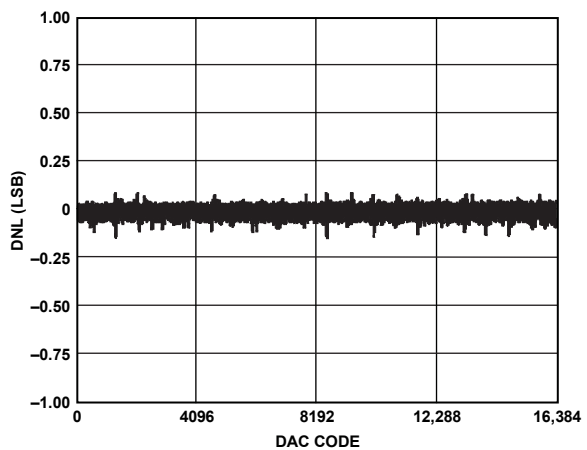
Figure 11. AD5025 DNL
