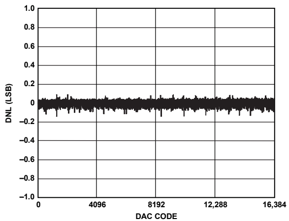
Figure 10. AD5045 DNL
