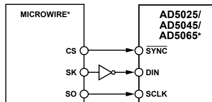
Figure 49. AD5025/AD5045/AD5065 to MICROWIRE Interface
