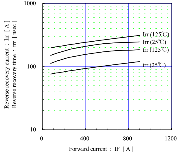
Reverse recovery characteristics (typ.) V cc =300V, V GE =±15V, R g =4.7Ω
