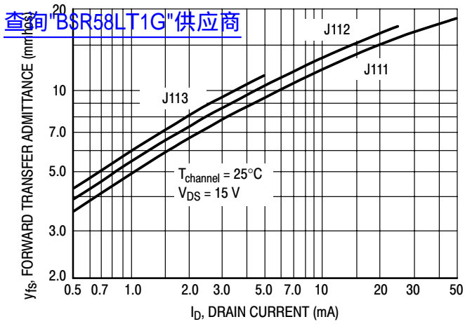
Figure 6. Typical Forward Transfer Admittance
