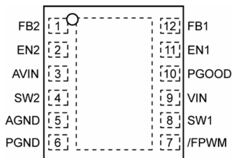
MIC2238-xxYML 12-Lead MLF ® (ML) (Top View)
