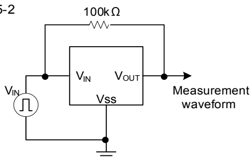
N-channel Open Drain Output
