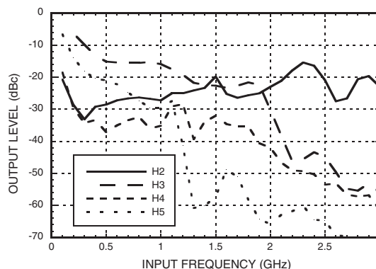
Divide-by-4 Harmonics [2], (Single-Ended)
