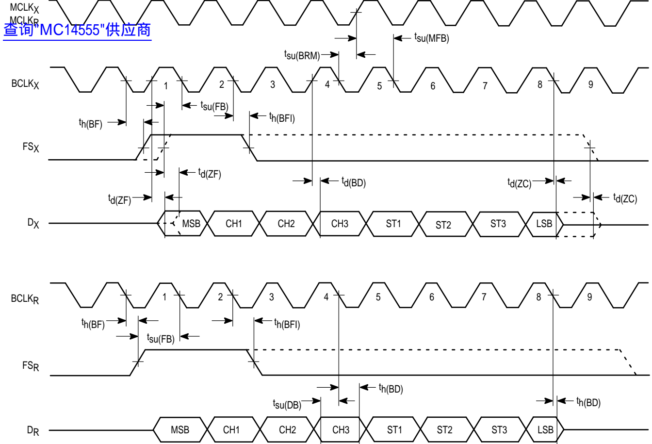
Figure 2. Long Frame Sync Timing
