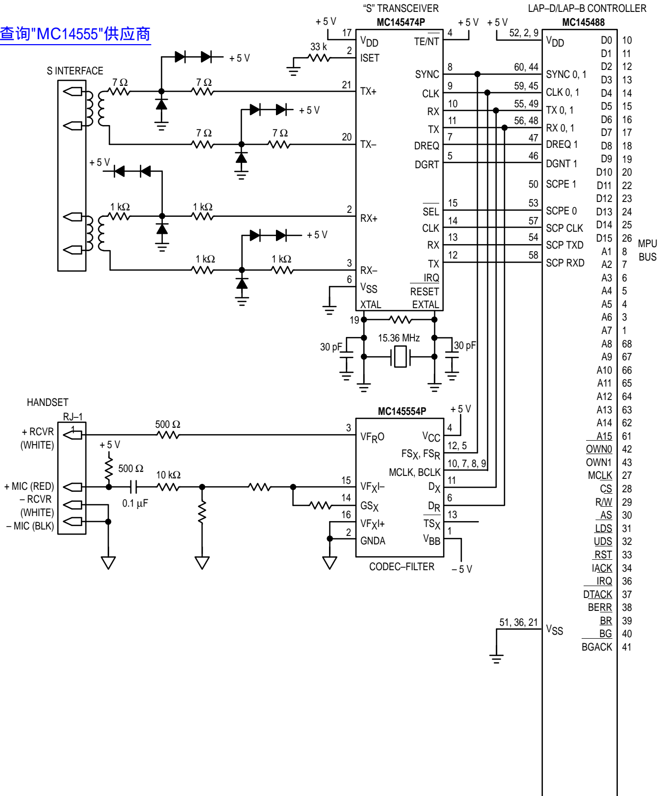
Figure 5. ISDN Voice/Data Terminal
