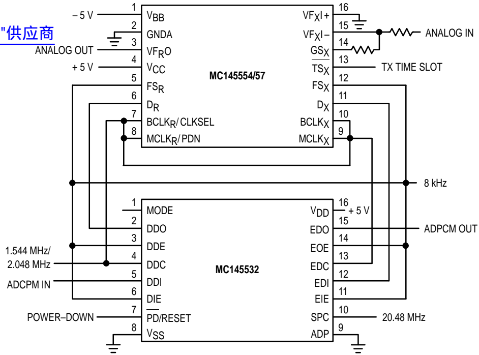
Figure 3. ADPCM Transcoder Application
