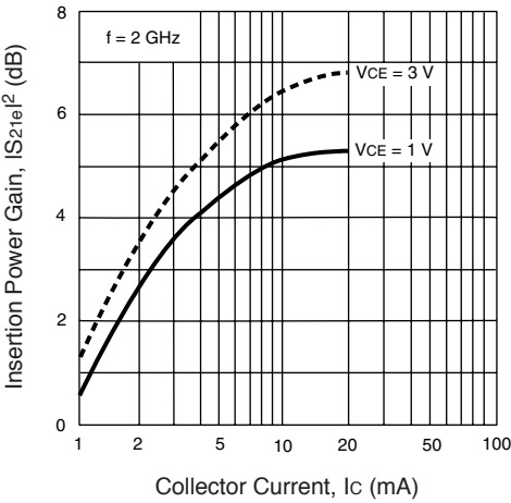
INSERTION GAIN vs. COLLECTOR CURRENT
