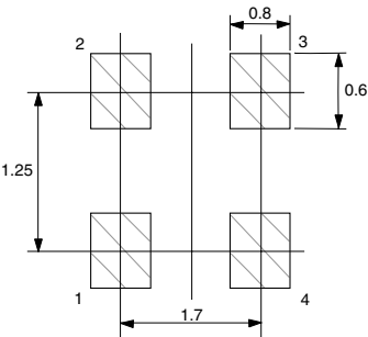
OUTLINE 19 RECOMMENDED P.C.B. LAYOUT
