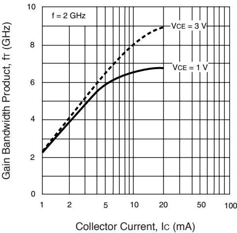
NE68839 GAIN BANDWIDTH PRODUCT vs. COLLECTOR CURRENT
