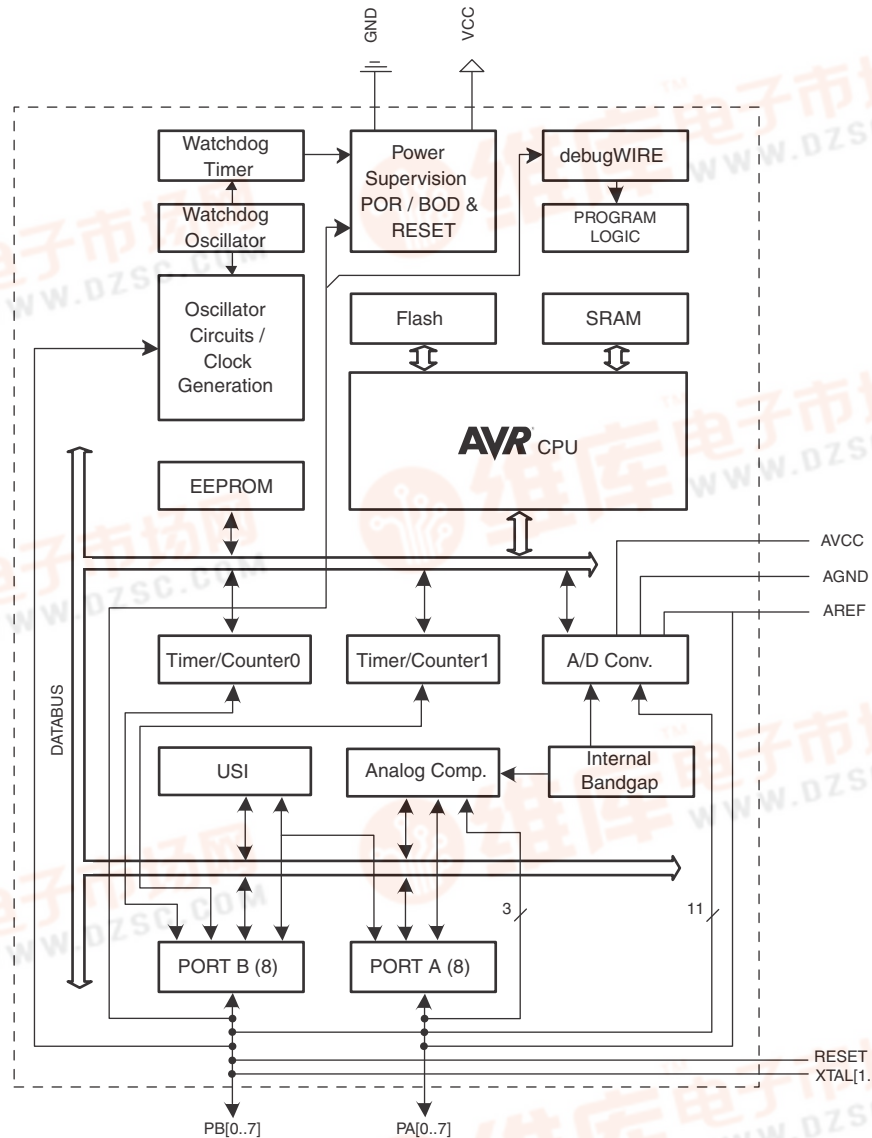
Figure 2-1. Block Diagram
