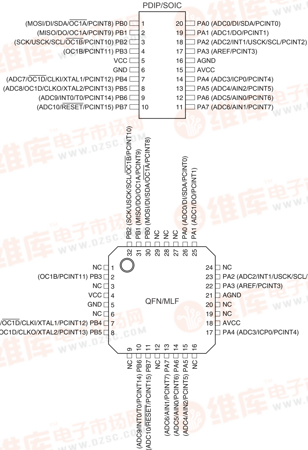
Figure 1-1. Pinout ATtiny261/461/861 and ATtiny261V/461V/861V
