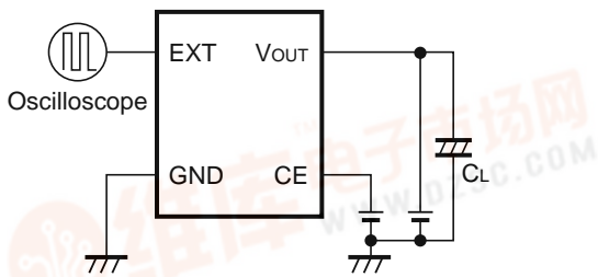
Test Circuit 3
