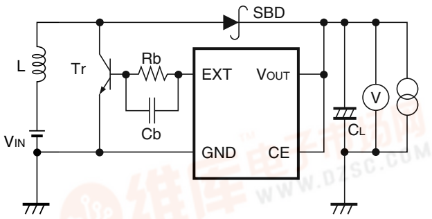
Test Circuit 1
