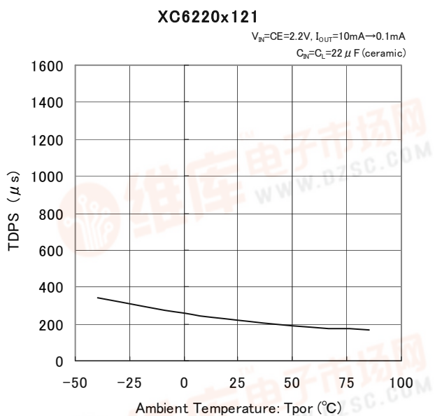
(6) PS Switching Delay Time vs. Ambient Temperature
