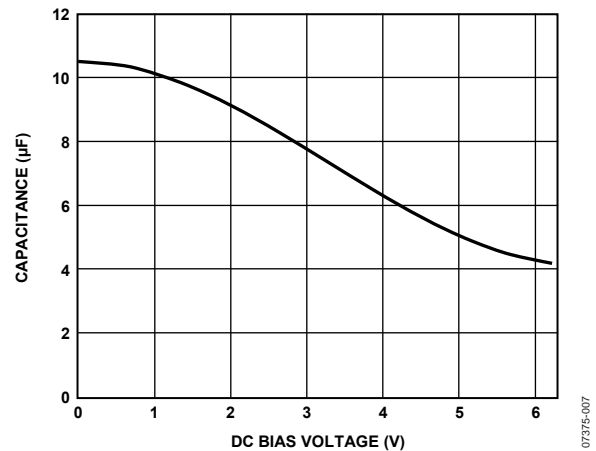
Figure 29. Typical Capacitor Performance
