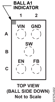
Figure 2. Pin Configuration
