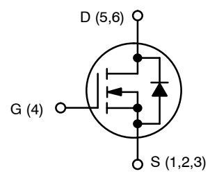
N-CHANNEL MOSFET
