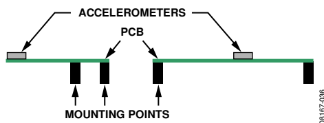
Figure 37. Incorrectly Placed Accelerometers
