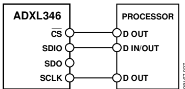
Figure 27. 3-Wire SPI Connection Diagram
