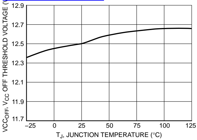
Figure 3. V CC OFF Threshold Voltage vs. Junction Temperature
