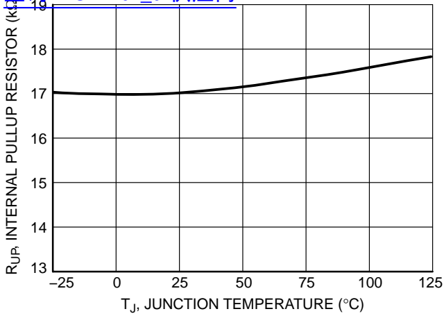
Figure 21. FB Pin Pullup Resistor vs. Junction Temperature
