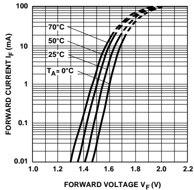
Figure 14. Typical Forward Current vs. Forward Voltage, HCPL-3101.
