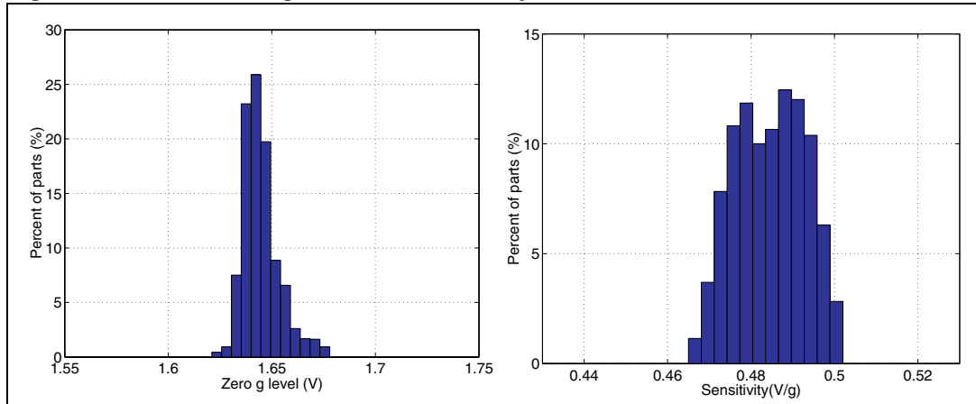
Figure 5. X-axis Zero-g level and Sensitivity at 3.3V
