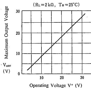
Maximum Output Voltage vs. Operating Voltage
