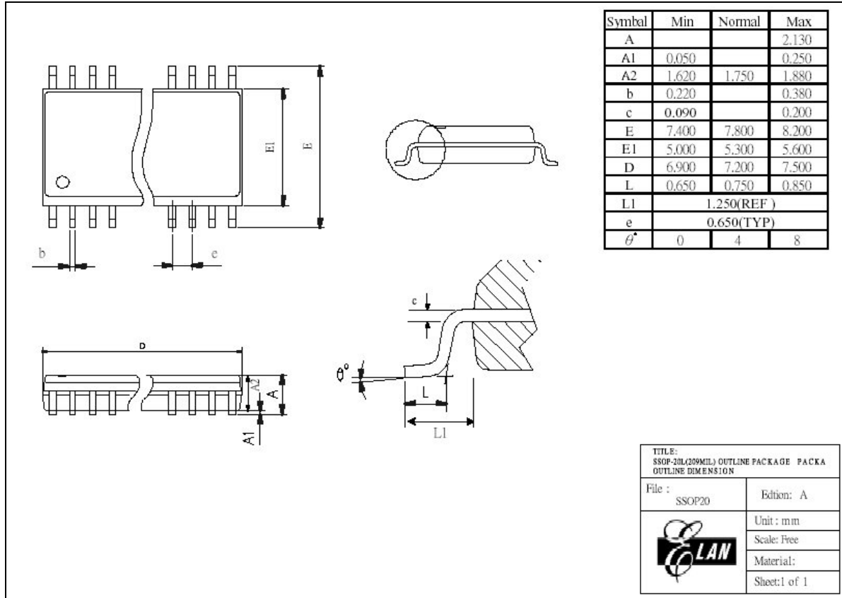
Figure B-5 EM78P346N 20-pin SSOP Package Type
