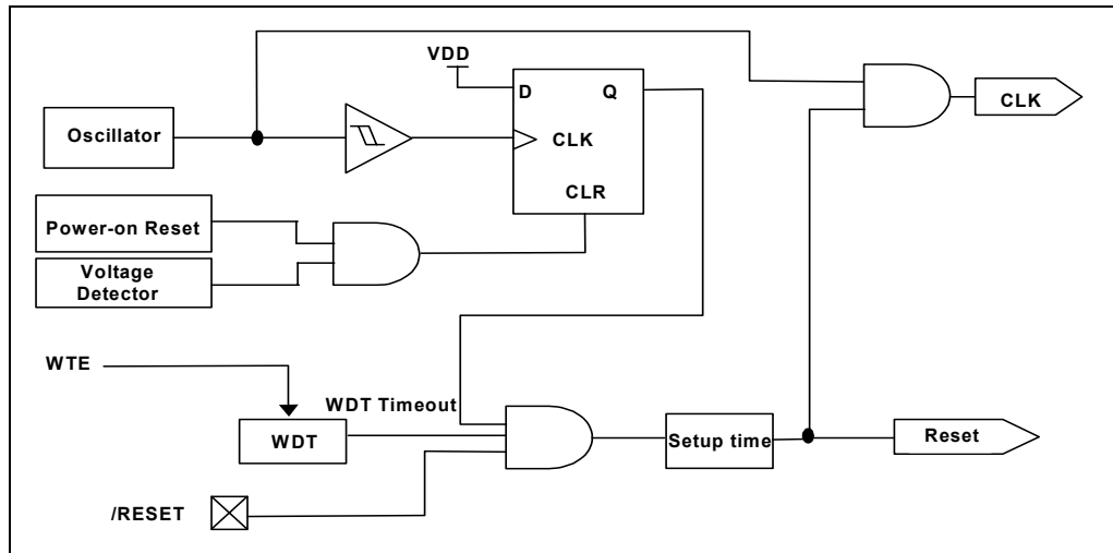
Figure 6-8 Controller Reset Block Diagram
