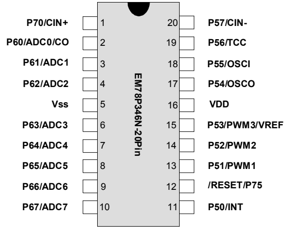
Figure 3-2 EM78P346ND20/SO20/SS20
