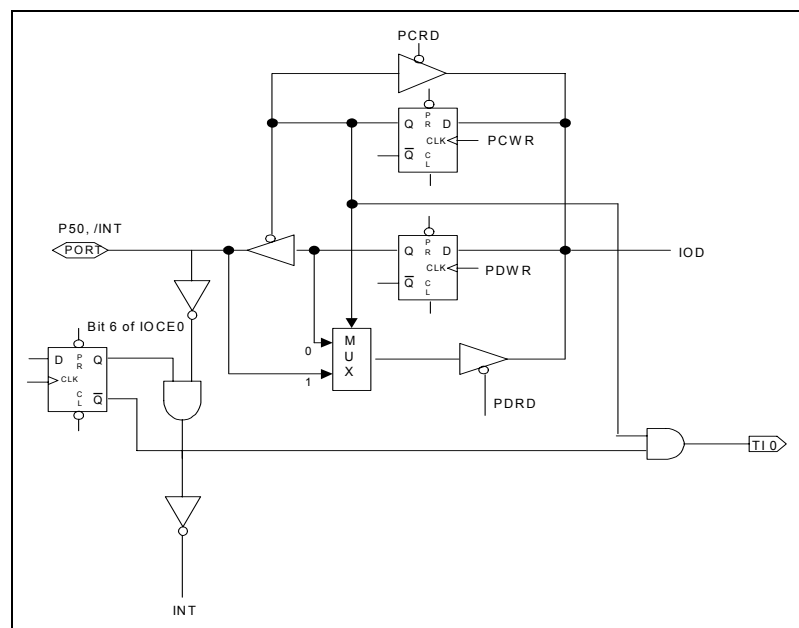
Figure 6-4 I/O Port and I/O Control Register Circuit for Port 5 and Port 6
