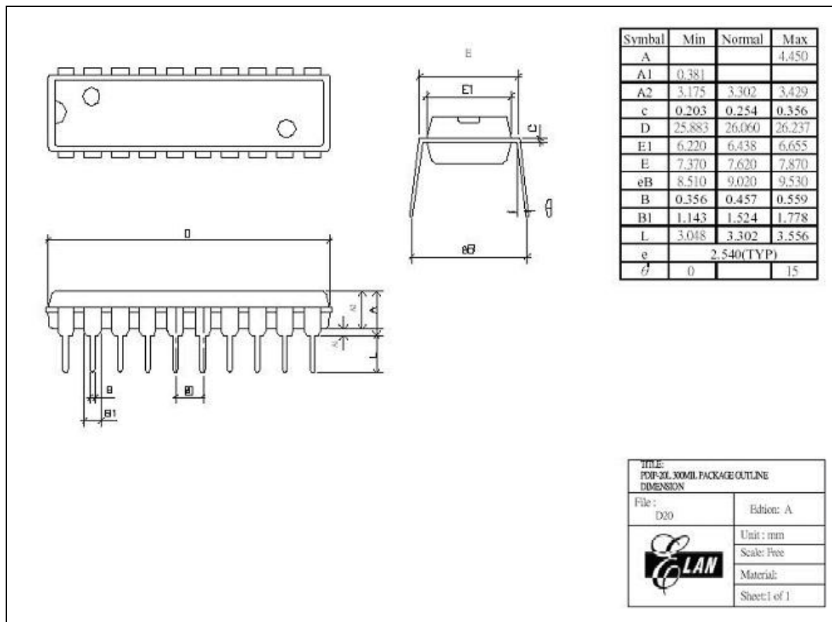
Figure B-3 EM78P346N 20-pin DIP Package Type
