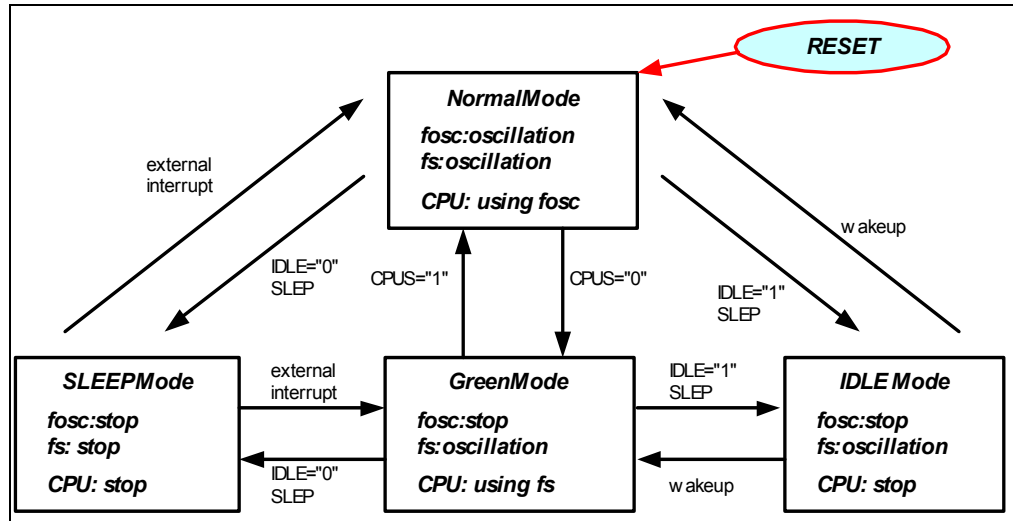
Figure 6-2 CPU Operation Mode
