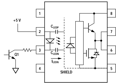
Figure 31. Not Recommended Open Collector Drive Circuit
