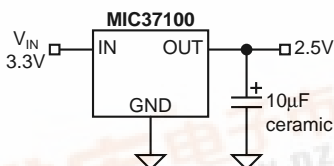
2.5V/1A Regulator
