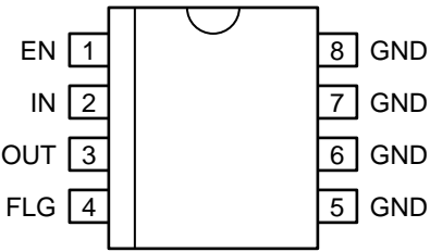
MIC37101-x.x (Fixed) SOIC-8 (M)
