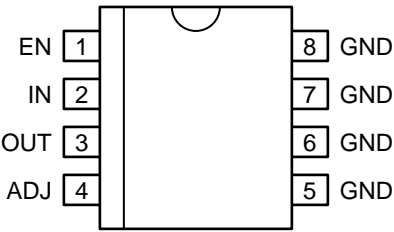
MIC37102 (Adjustable) SOIC-8 (M)
