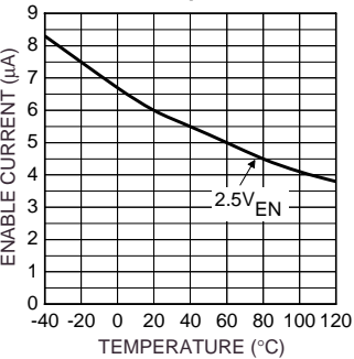
Enable Current vs. Temperature
