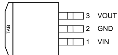
S-PAK-3 (R)
