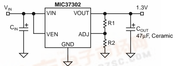
Adjustable Regulator
