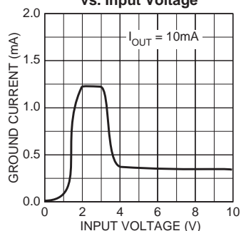
MIC2931x Ground Current vs. Input Voltage
