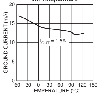
MIC2931x Ground Current vs. Temperature
