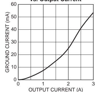
MIC2931x Ground Current vs. Output Current
