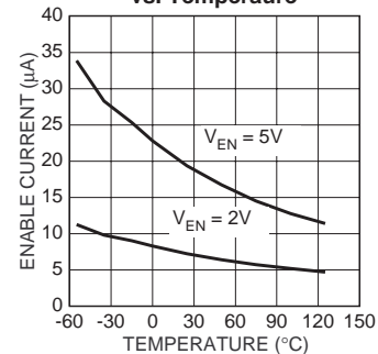
MIC29312 Enable Current vs. Temperature
