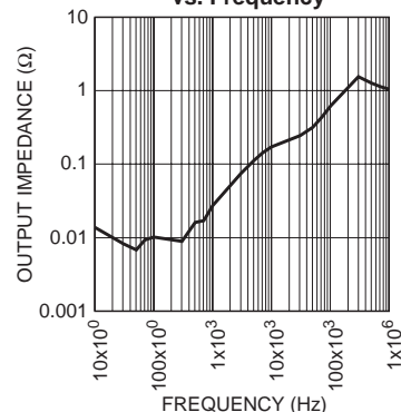
MIC2931x Output Impedance vs. Frequency
