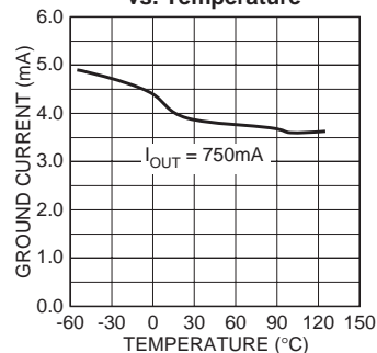
MIC2931x Ground Current vs. Temperature
