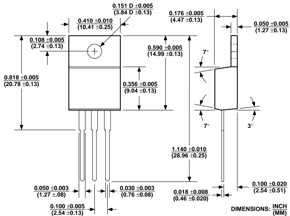
TO-220-3 (T)
