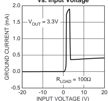
MIC2931x Ground Current vs. Input Voltage
