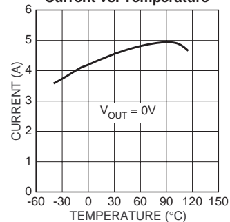
MIC2931x Short Circuit Current vs. Temperature
