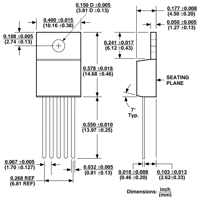
TO-220-5 (T)
