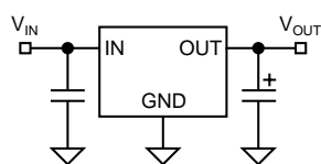
Figure 3. The MIC29310 regulator requires only two capacitors for operation.
