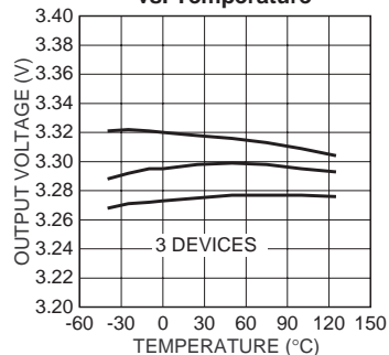
MIC29310-3.3 Output Voltage vs. Temperature
