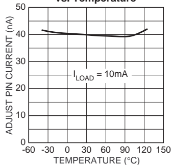
MIC29312 Adjust Pin Current vs. Temperature
