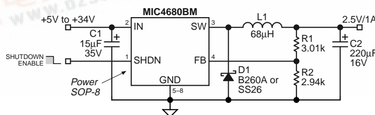
Adjustable Regulator Circuit
