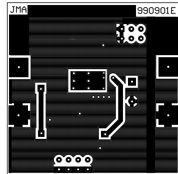
Figure 6e. Bottom-Side Copper
