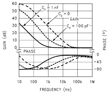
16.8V Bode Plot
