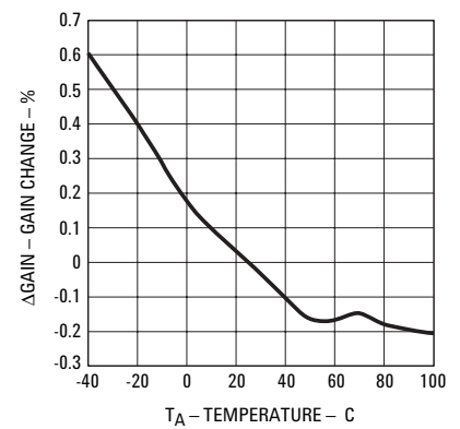
Figure 9. Gain change vs. temperature.
