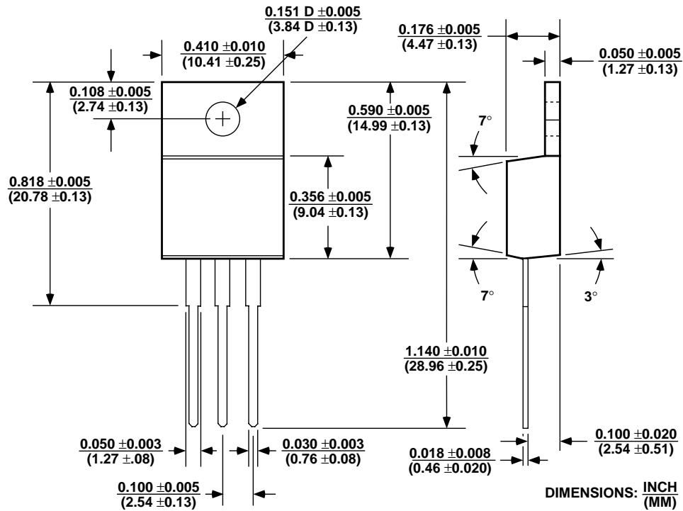
TO-220-3 (T)
