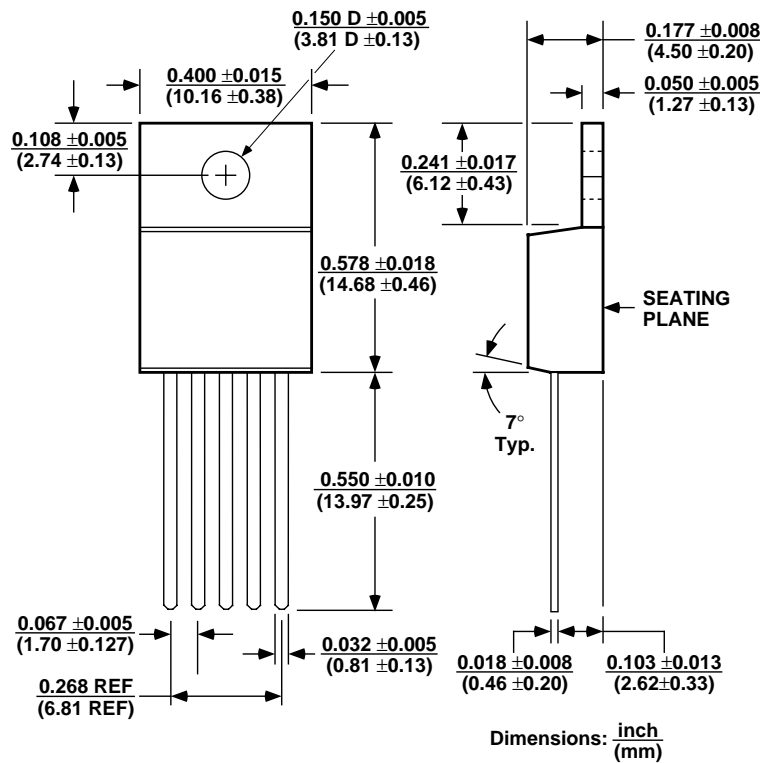
TO-220-5 (T)
