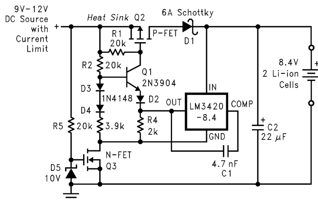
FIGURE 11. MOSFET Low Dropout Charger
