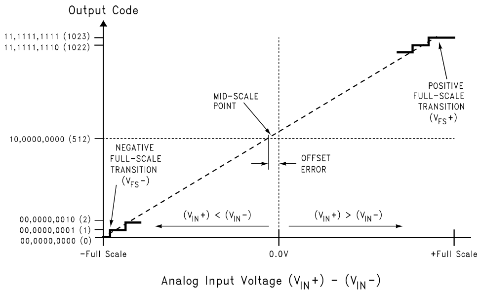
FIGURE 2. Input vs. Output Transfer Characteristic
