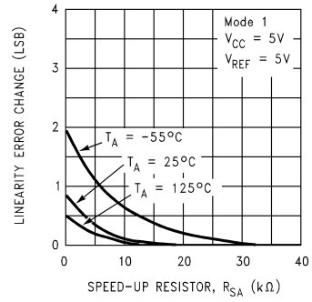
Linearity Change vs Speed-Up Resistor (ADC10062 and ADC10064 Only)
