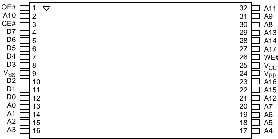
32-Pin TSOP—Reverse Pinout
