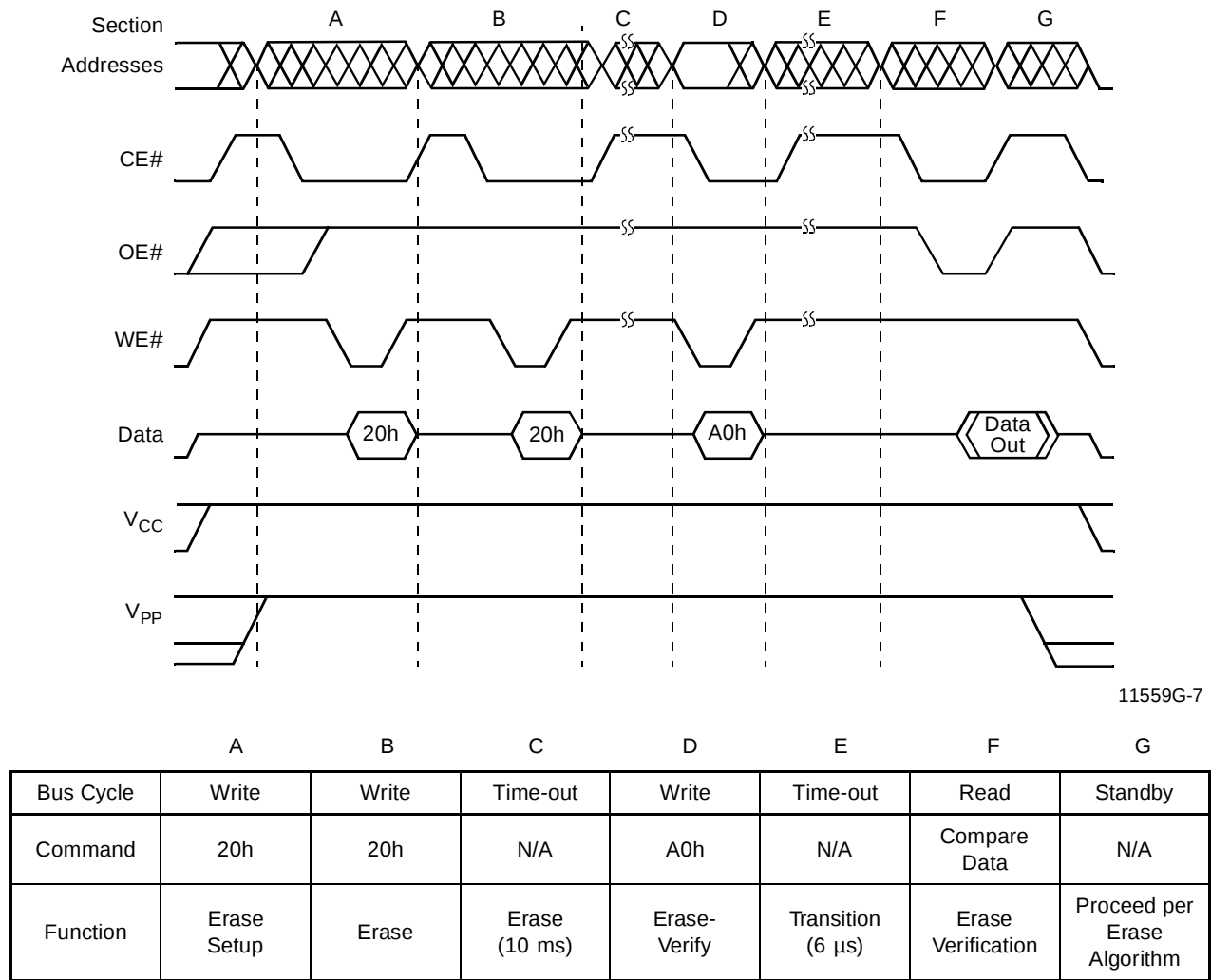
Figure 2. AC Waveforms For Erase Operations
