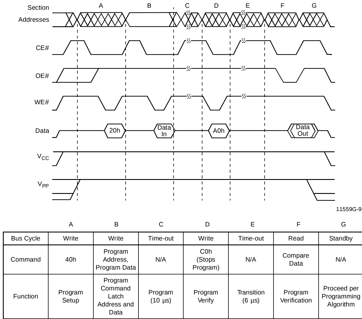
Figure 4. AC Waveforms for Programming Operations
