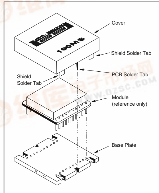
FIGURE 2. Assembly Diagram.
