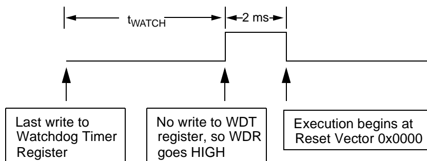
Figure 7-1. Watchdog Reset (Address 0x26)
