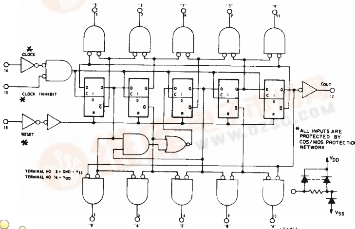
Fig. 1 - Logic diagram.
