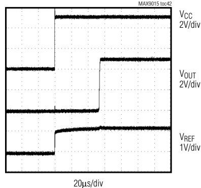
POWER-UP RESPONSE
