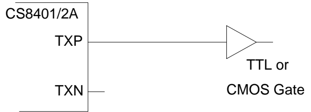
Figure A3. TTL/CMOS Output Circuit
