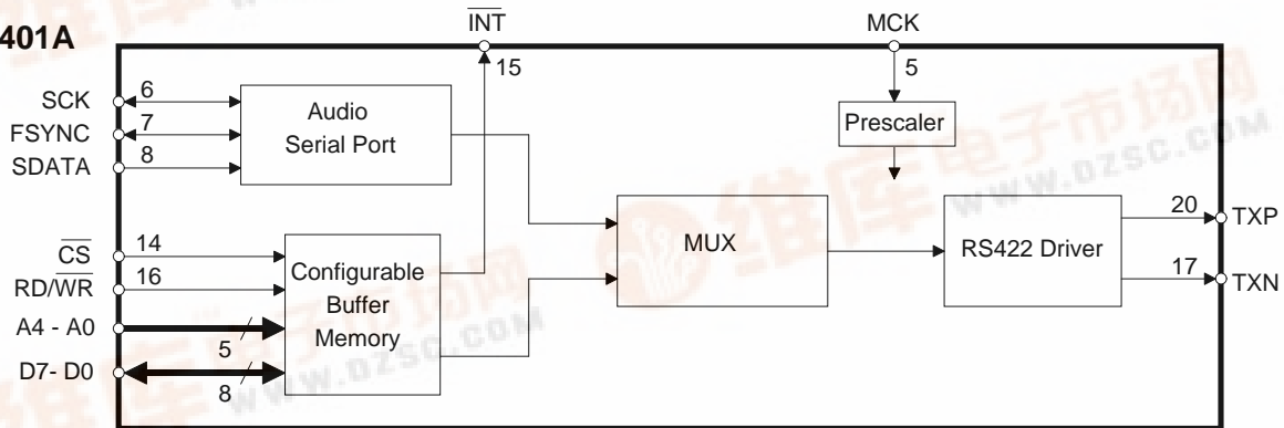
CS8402A
