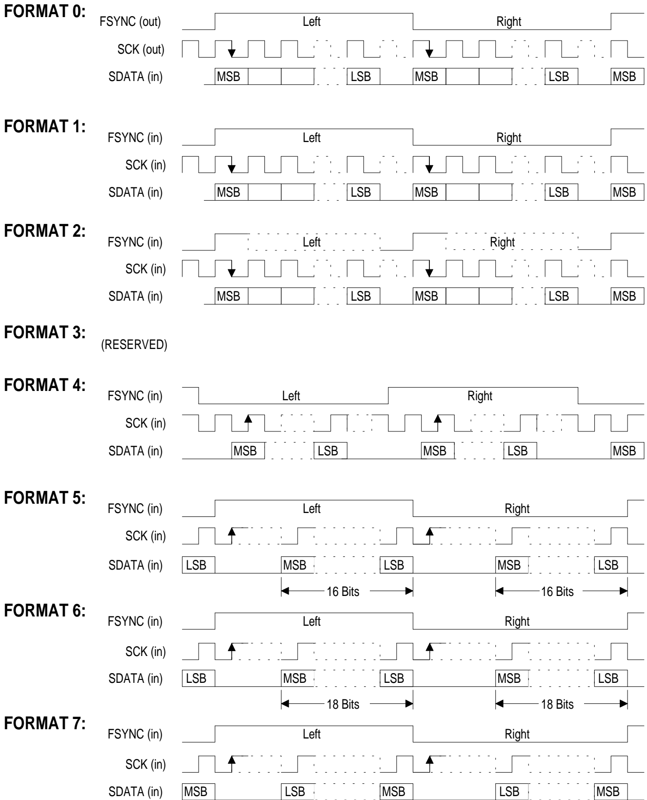
Figure 16. CS8402A Audio Serial Port Formats
