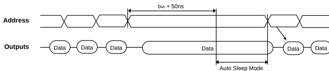
Figure 3. Auto Sleep Mode Operation
