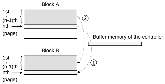
Figure 25. Block Replacement
