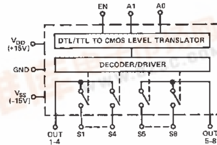
AD7502
