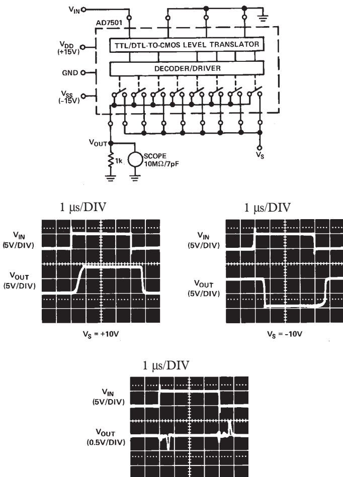
TEST CIRCUIT 2
