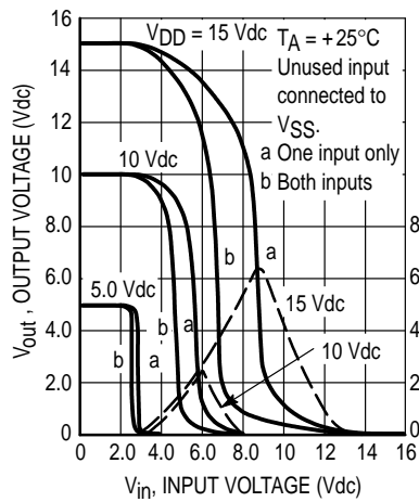
Figure 2. Typical Voltage and Current Transfer Characteristics
