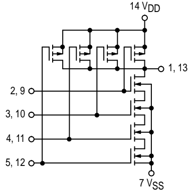
MC14012UB CIRCUIT SCHEMATIC (1/2 of Device Shown)
