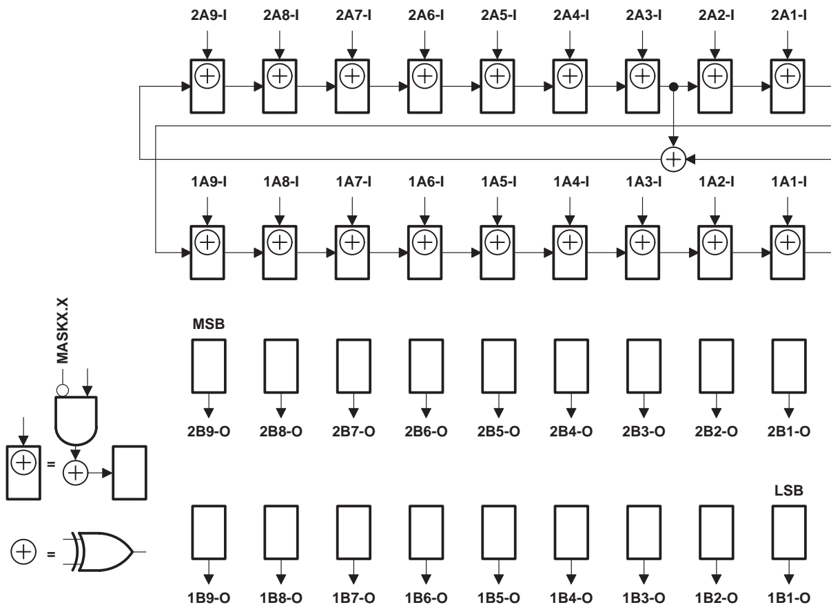
Figure 10. 18-Bit PSA/COUNT Configuration (1OEAB = 2OEAB = 0, 1OEBA = 2OEBA = 1)
