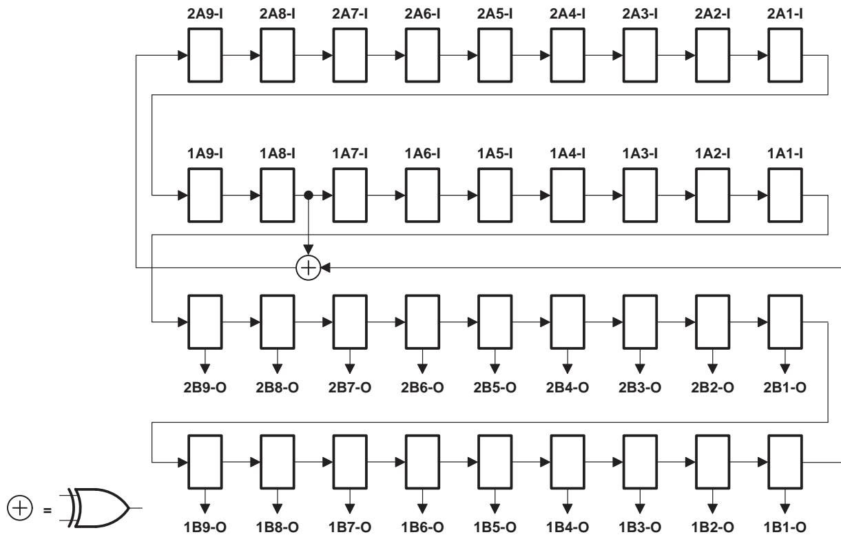
Figure 4. 36-Bit PRPG Configuration (1OEAB = 2OEAB = 0, 1OEBA = 2OEBA = 1)
