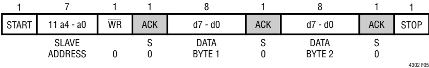
Figure 5. Writing Two Bytes
