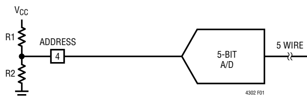
Figure 1. Address Compare Circuitry
