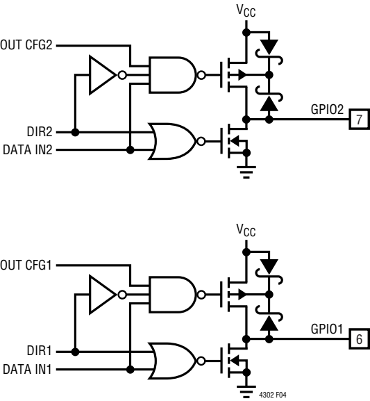
Figure 4. GPIO Circuits and Their Control Bits
