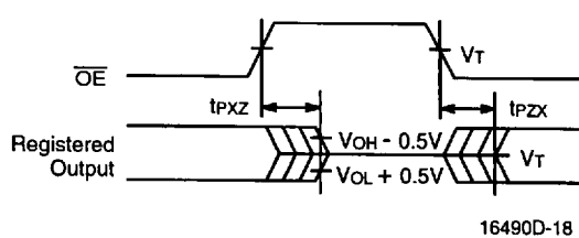
\overline{\text{OE}} to Output Disable/Enable
