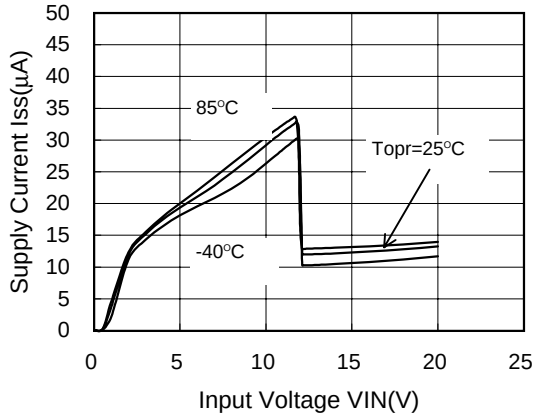
XC6202PC02 (12V)
