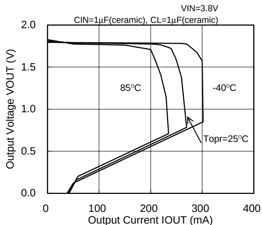
XC6202P182(1.8V)
