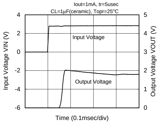
XC6202P182(1.8V)
