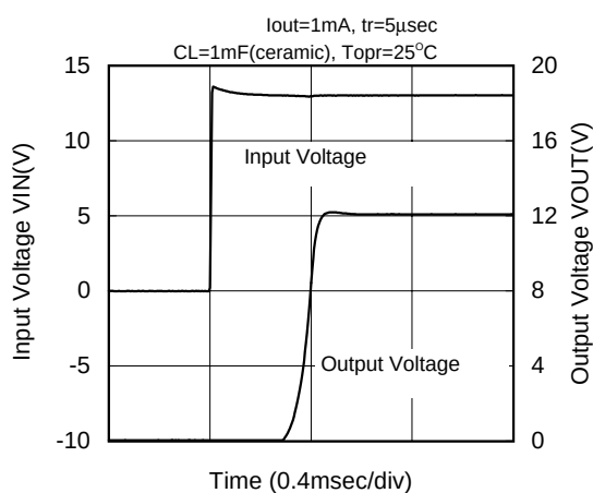
XC6202PC02 (12V)
