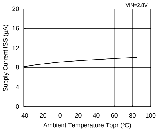
XC6202P182(1.8V)
