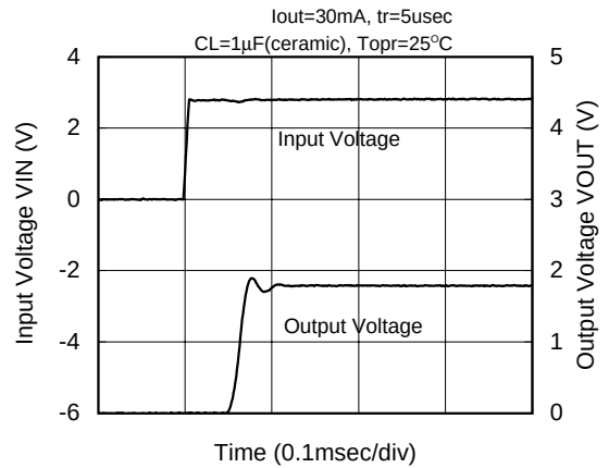
XC6202P182(1.8V)
