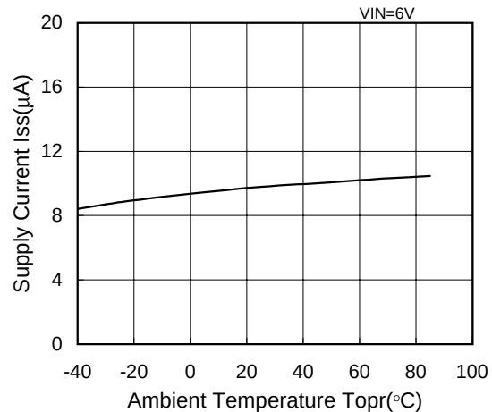
XC6202P502 (5V)
