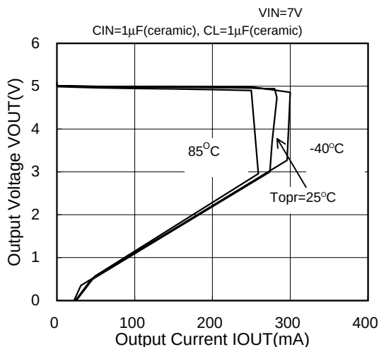
XC6202P502 (5V)
