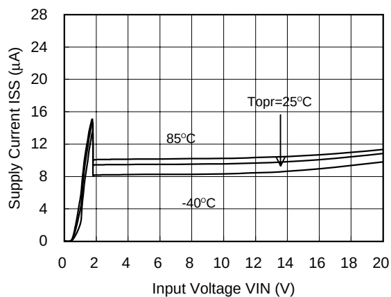
XC6202P182(1.8V)
