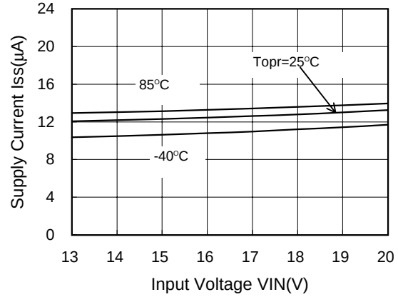
XC6202PC02 (12V)
