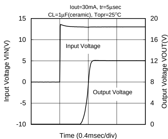
XC6202PC02 (12V)
