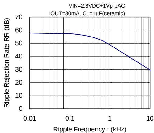
XC6202P182(1.8V)
