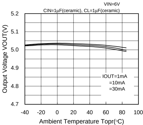
XC6202P502 (5V)
