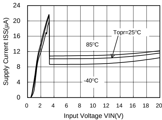
XC6202P332(3.3V)
