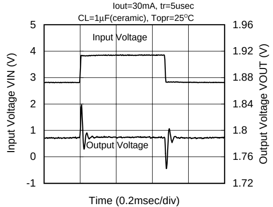
XC6202P182(1.8V)
