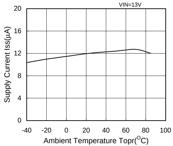
XC6202PC02 (12V)
