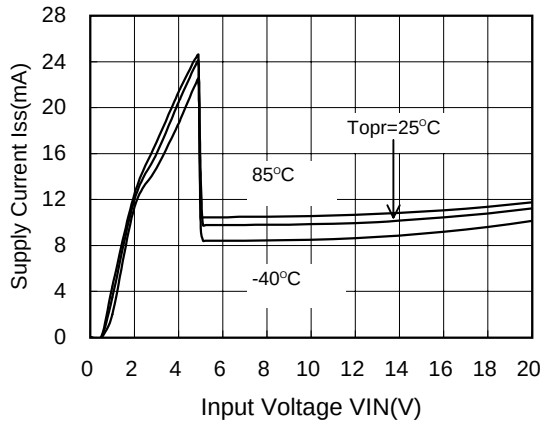
XC6202P502 (5V)
