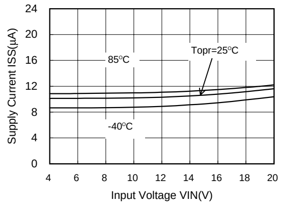
XC6202P332(3.3V)
