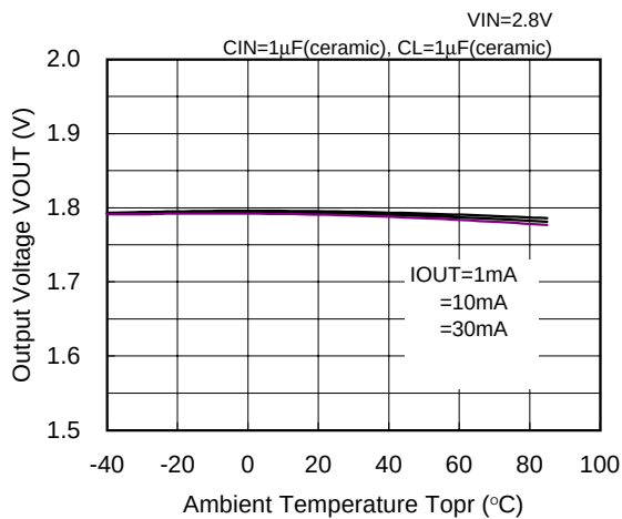
XC6202P182(1.8V)
