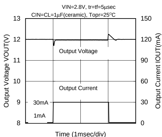
XC6202PC02 (12V)
