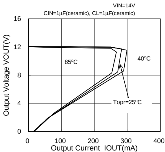
XC6202PC02 (12V)
