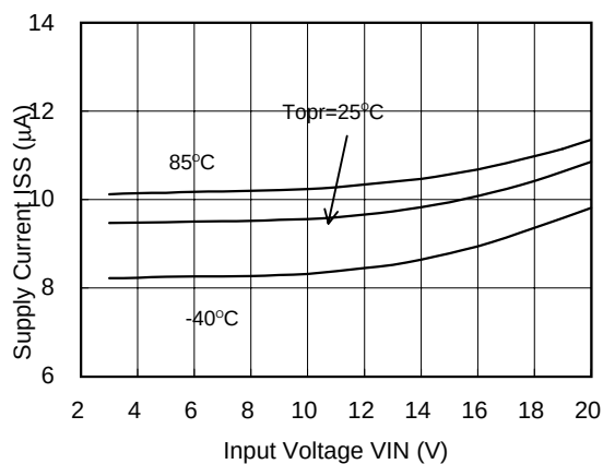
XC6202P182(1.8V)
