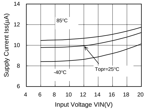
XC6202P502 (5V)
