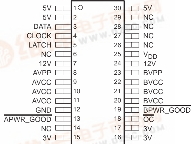
DB OR DF PACKAGE (TOP VIEW)
