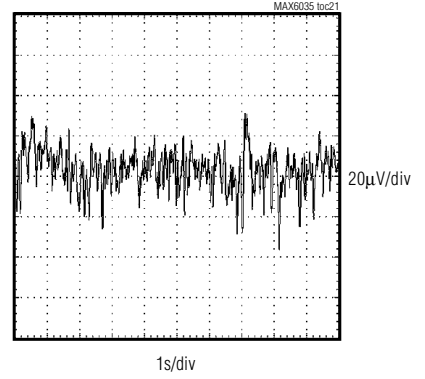
MAX6035 0.1Hz to 10kHz OUTPUT NOISE ( V_{OUT} = 5V )
