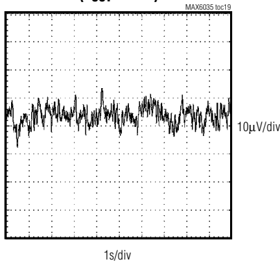
MAX6035 0.1Hz to 10kHz OUTPUT NOISE ( V_{OUT} = 2.5V )
