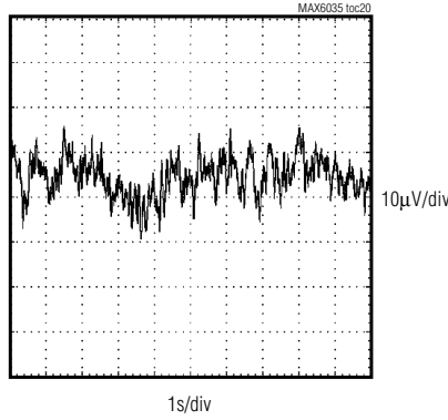
MAX6035 0.1Hz to 10kHz OUTPUT NOISE ( V_{OUT} = 3V )
